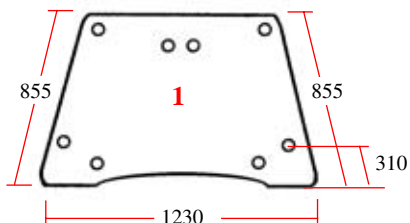
25/4004-1 (D.7091, 144986A1) Parabrisas 8 agujeros Windscreen 8 holes
