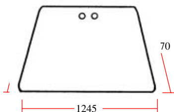
25/4000-48 (D.7090, 144768A1) Parabrisas 2 agujeros Windscreen 2 holes
