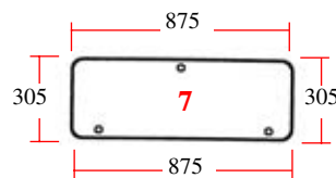
25/4073-14 (D.7018, 3233032R1) Trasero (inferior) Rear (lower)
