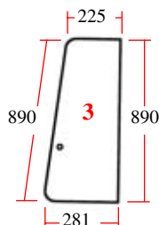
25/4026-2 (D.7013, 3233053R1) Puerta (delantera) Door (front)
