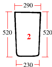
25/4012-23 (D.7011, 3233036R1) Delantero inferior (Drcha & Izq) Front (RH & LH)
