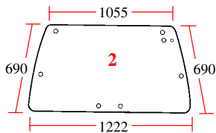
20/4072-26 (D7029, K312000) Trasero 8 agujeros Rear 8 holes
