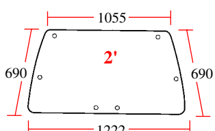
20/4072-27 (D7029/A, K303696) Trasero 6 agujeros Rear 6 holes
