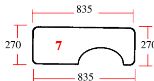
25/4073-15 (D.7019, 1500941C1) Trasero (inferior) Rear (lower)
