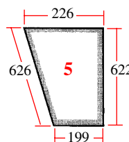
25/4037-1 (D.7046, 3125459R1) Puerta (inferior izq.) Door (LH lower)
