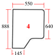
25/4027-2 (D.7014, 3233051R1) Puerta (fijo) Door
