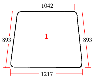
25/4000-36 (D.7010, 3233045R1) Parabrisas Windscreen
