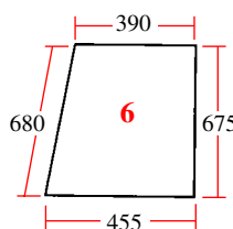
25/4041-5 (D.7048/F, 3125392R1)) Fijo (izq. o drcha.) Side fixed (LH & RH)
