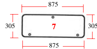
25/4073-14 (D.7018, 3233032R1) Trasero (inferior) Rear (lower)
