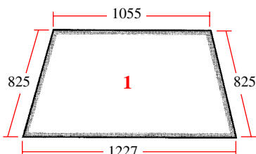
25/4002-2 (D.7040, 3125386R1) Marco + Parabrisas Frame + windscreen
