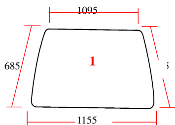
25/4000-35 (D.7000, 3113554R1) Parabrisas Windscreen
