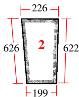
25/4015-2 (D.7042, 3125387R1) Delantera (izq.) Front (LH)
