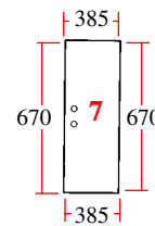
25/4040-3 (D.7048/S, 3125391R1) Deslizante (izq. o drcha.) Side sliding (LH & RH)
