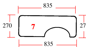
25/4073-15 (D.7019, 1500941C1) Trasero (inferior) Rear (lower)
