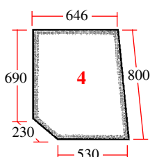
25/4034-1 (D.7043, 3125458R1) Puerta (superior drcha.) Door (RH upper)
