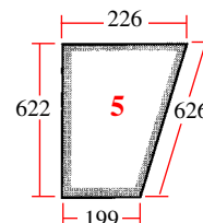
25/4036-1 (D.7045, 3125460R1) Puerta (superior drcha.) Door (RH lower)
