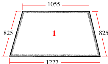
20/4002-2 (D7040, K965652) Soporte + Parabrisas Frame + windscreen
