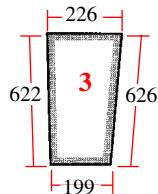
20/4016-2 (D7041, K965470) Delantera (dcha) Front (RH)
