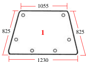
25/4000-45 (D7060, 1535093C2) Parabrisas Windscreen
