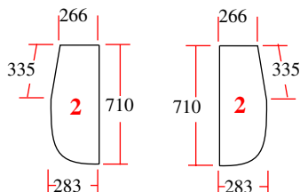
25/4012-24 (D.7001, 3113558R1) Delantero inferior (drcha. & izq.) Front (RH & LH)
