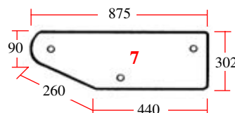
25/4073-21 (D7065, 1535071C1) Trasero (inferior) Rear (lower)
