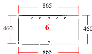
25/4073-12 (D.7005, 3118657R1) Trasero (inferior, 6 agujeros) Rear (lower, 6 holes)
