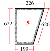
20/4036-1 (D7045, K965486) Puerta (inferior dcha) Door (RH lower)
