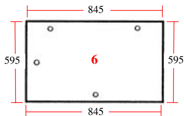
25/4072-32 (D7064, 1535079C1) Trasero (superior) Rear (upper)
