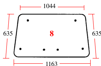
25/4041-5 (D.7048/F, 3125392R1)) Fijo (izq. o drcha.) Side fixed (LH & RH)
