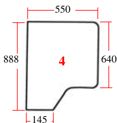
25/4027-2 (D.7014, 3233051R1) Puerta (trasera) Door (rear)
