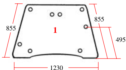
25/4004-3 (D.7091/A, 234969A1) Parabrisas 8 agujeros Windscreen 8 holes
